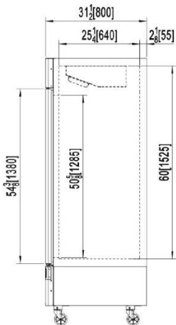
SIDE VIEW (1,2,3) DOOR MODELS
