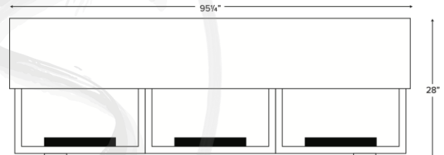
C-HBC95-HC TOP VIEW
