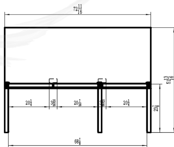
C-U72R-HC TOP VIEW
