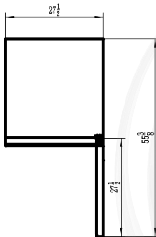
C-U27R-HC TOP VIEW
