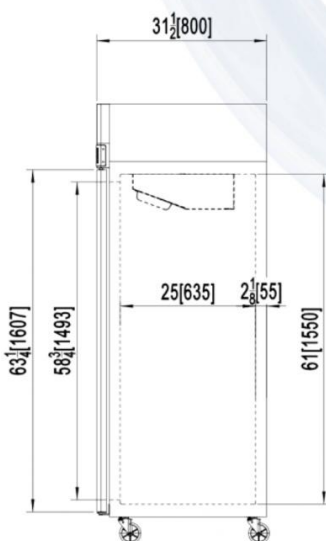
SIDE VIEW (1,2,3) DOOR MODELS
