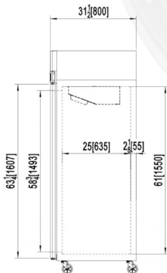
SIDE VIEW (1,2,3) DOOR MODELS
